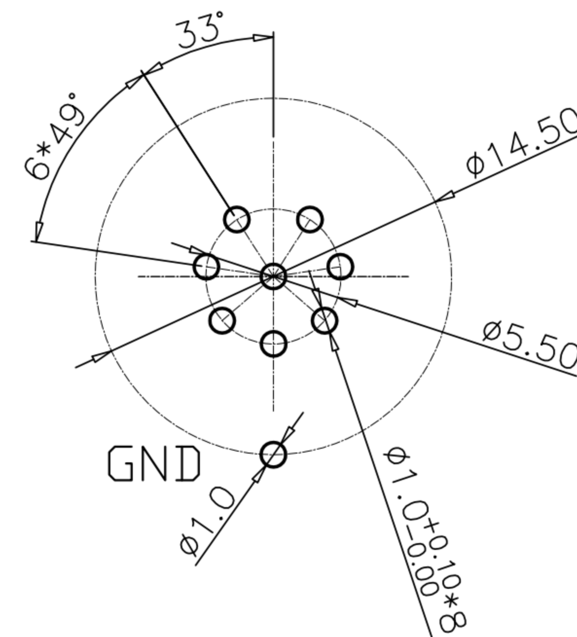
RECOMMEND PANEL CUT-OUT RECOMMEND P.C.B LAYOUT
