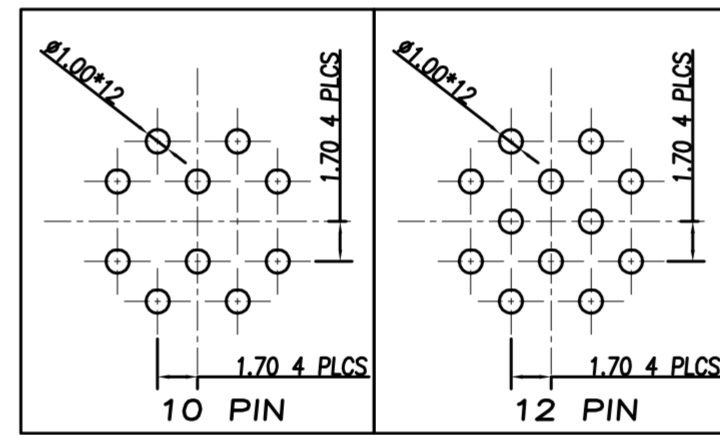
PCB LAYOUT
