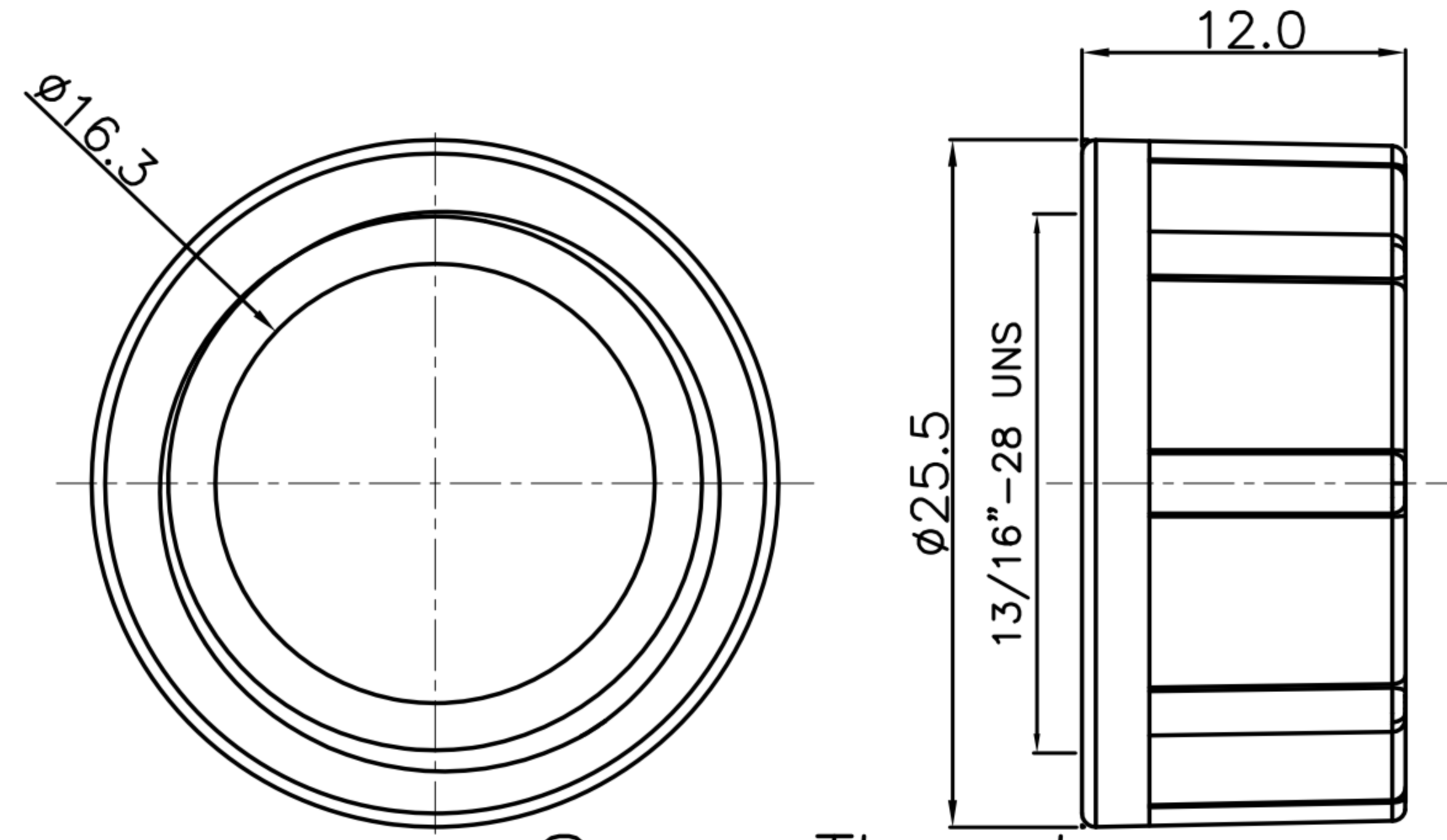
Screw Thread
