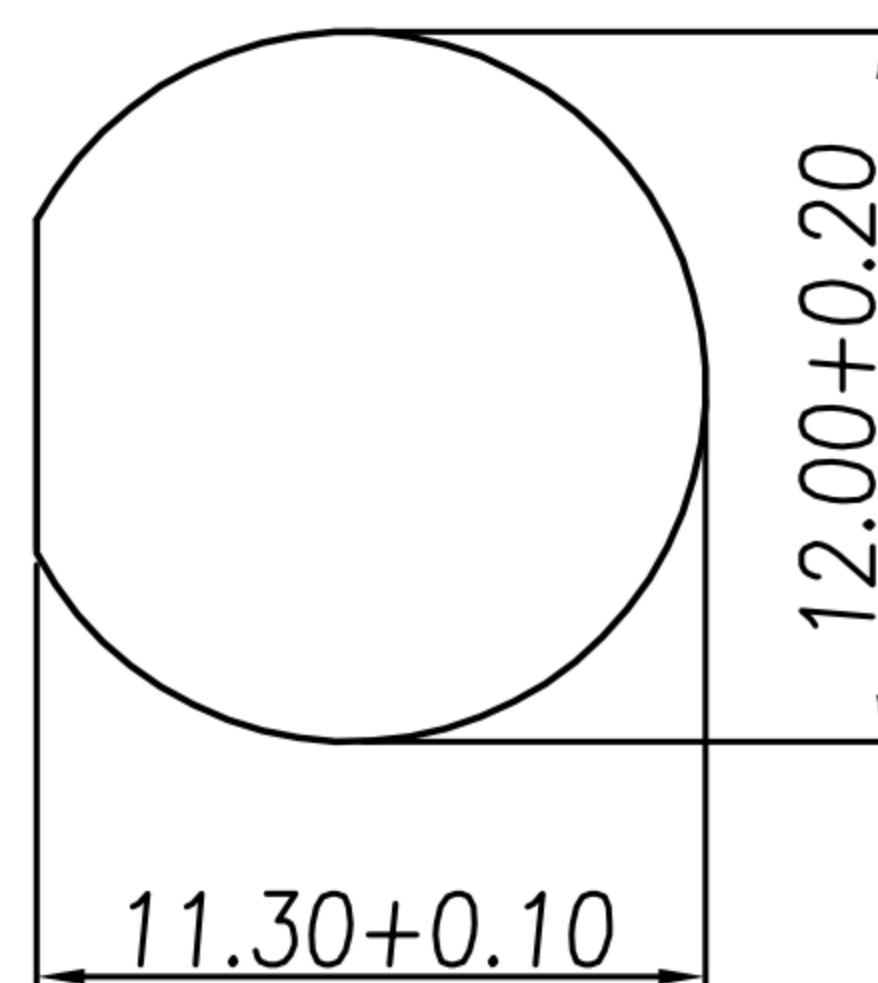
PANEL CUT-OUT
