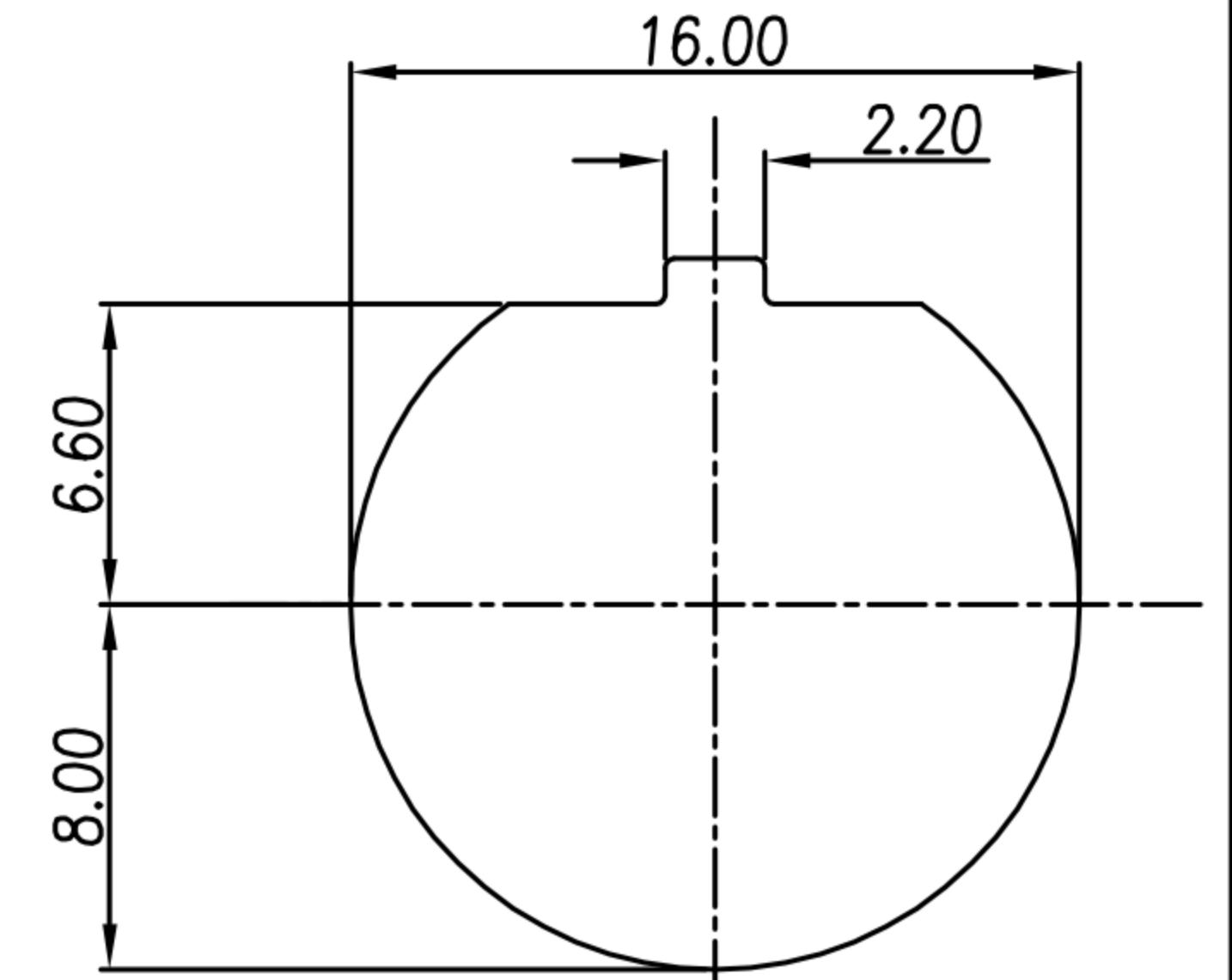
PANEL CUT-OUT
