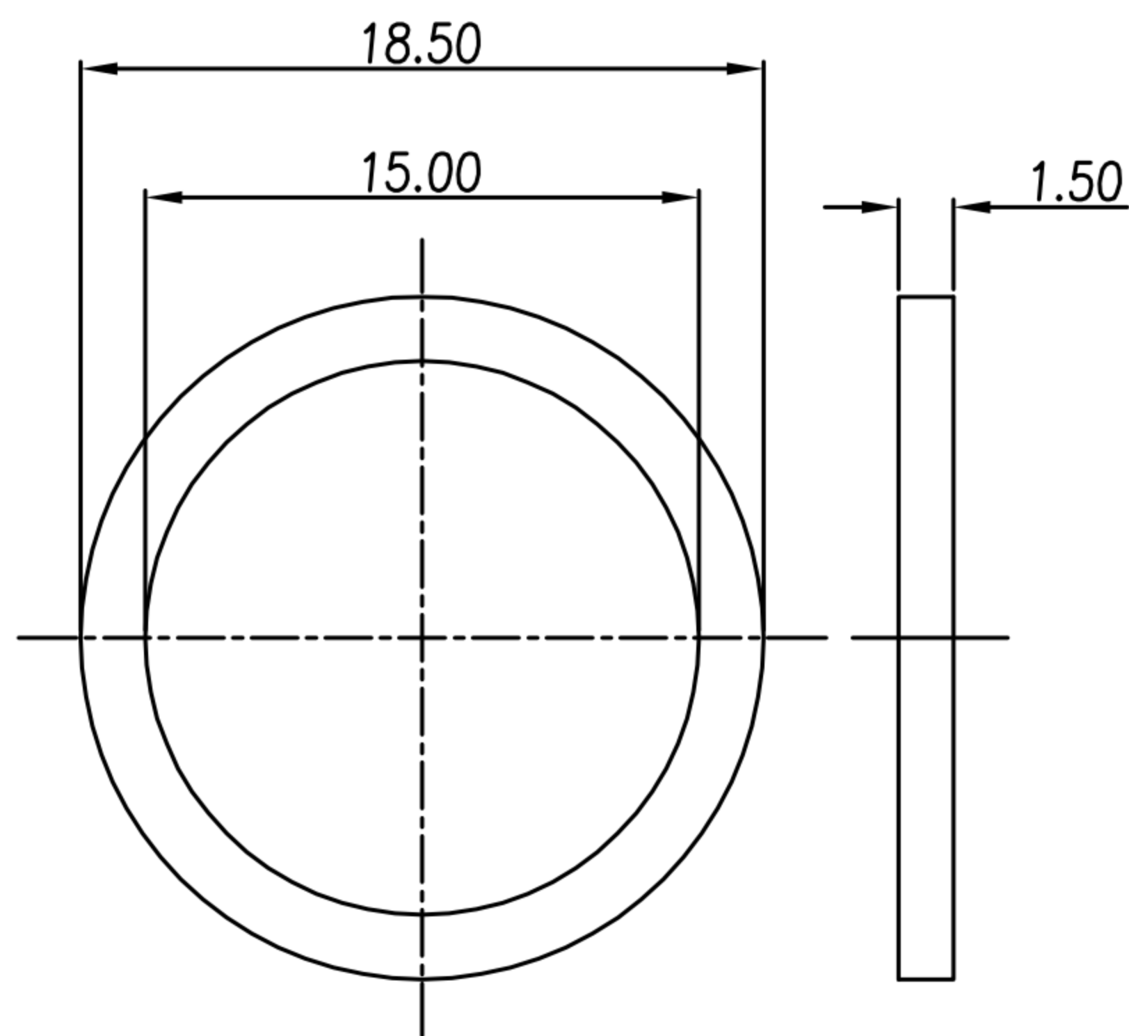
O-RING
