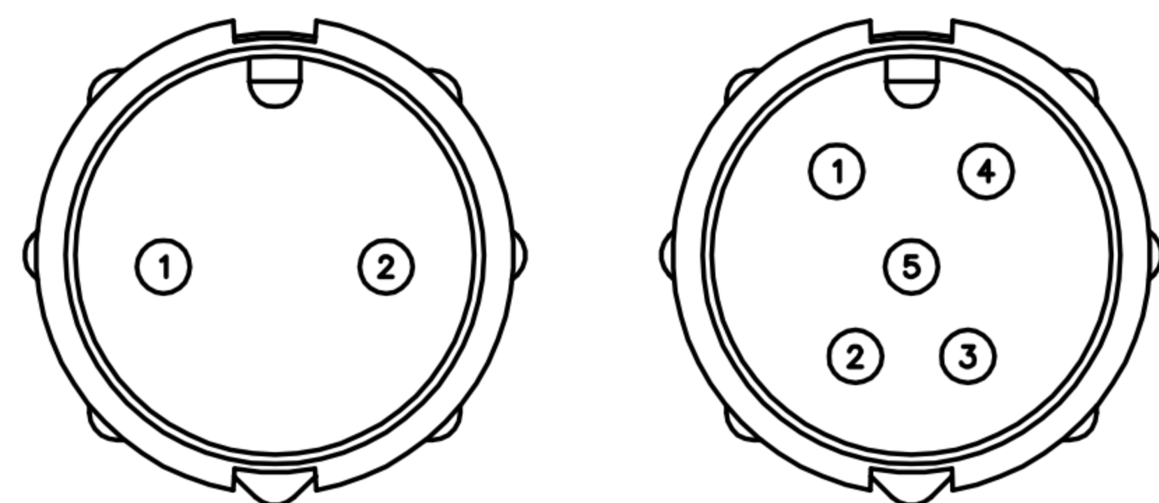
Pin Assignments Front View
