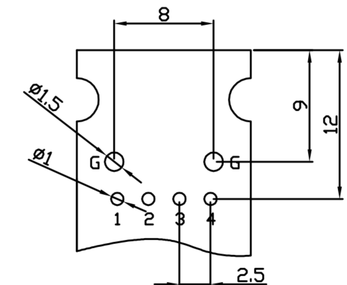
P.C.B LAYOUT TOP VIEW
