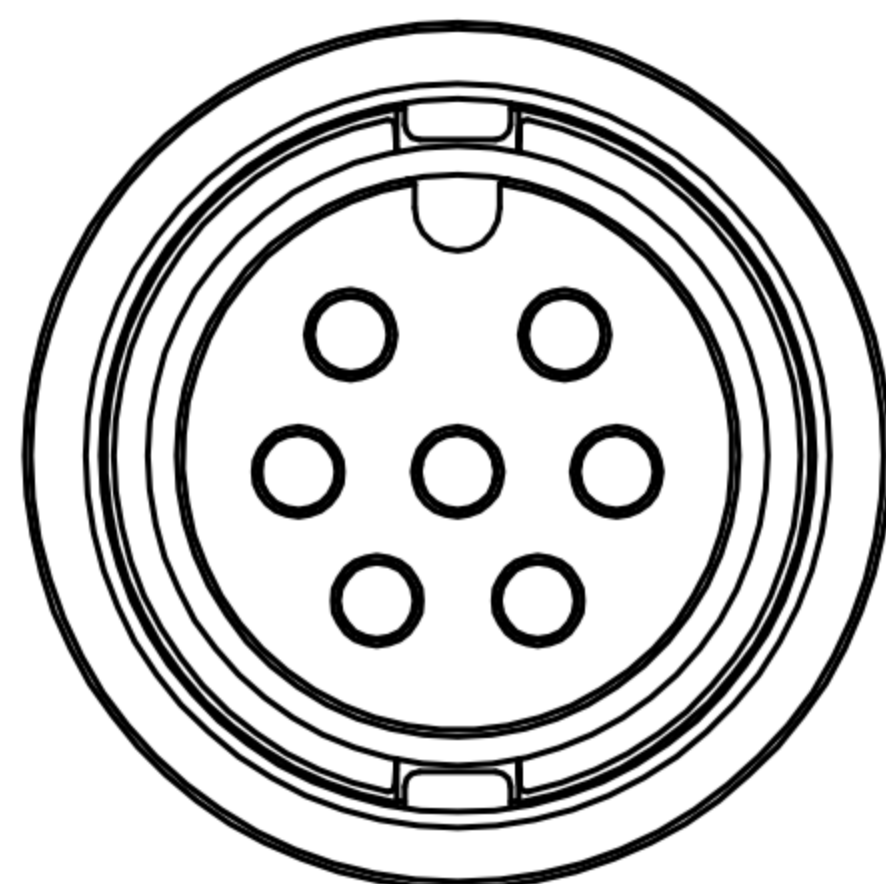
Pin Assignments Front View
