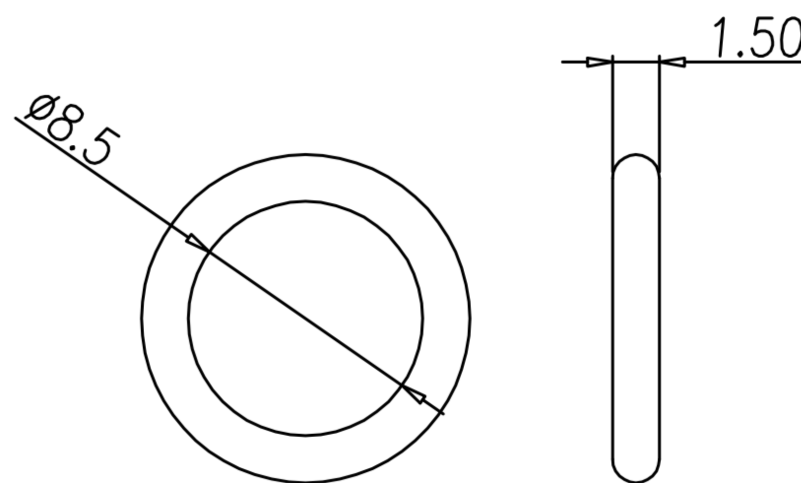
O-RING
