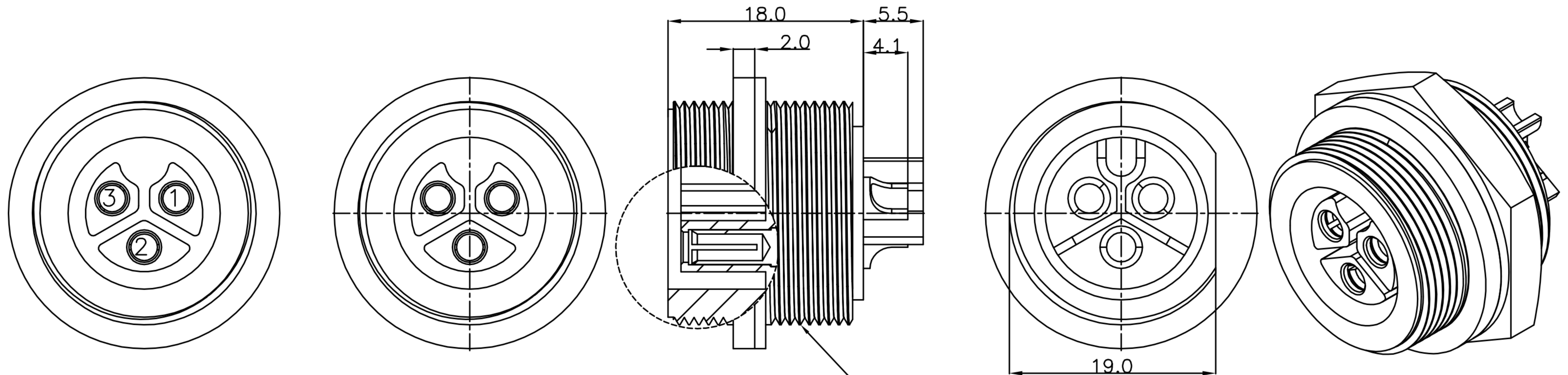
Pin Assignments Front View
