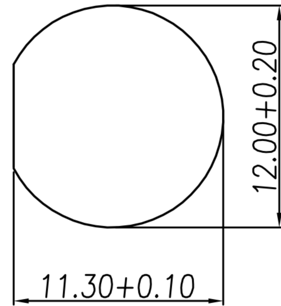
PANEL CUT-OUT
