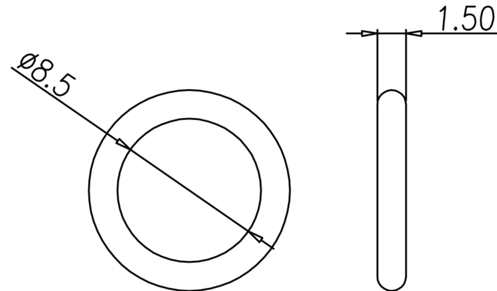
O-RING
