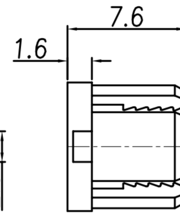
BACK SHELL+SHIELDING+O-RING2
