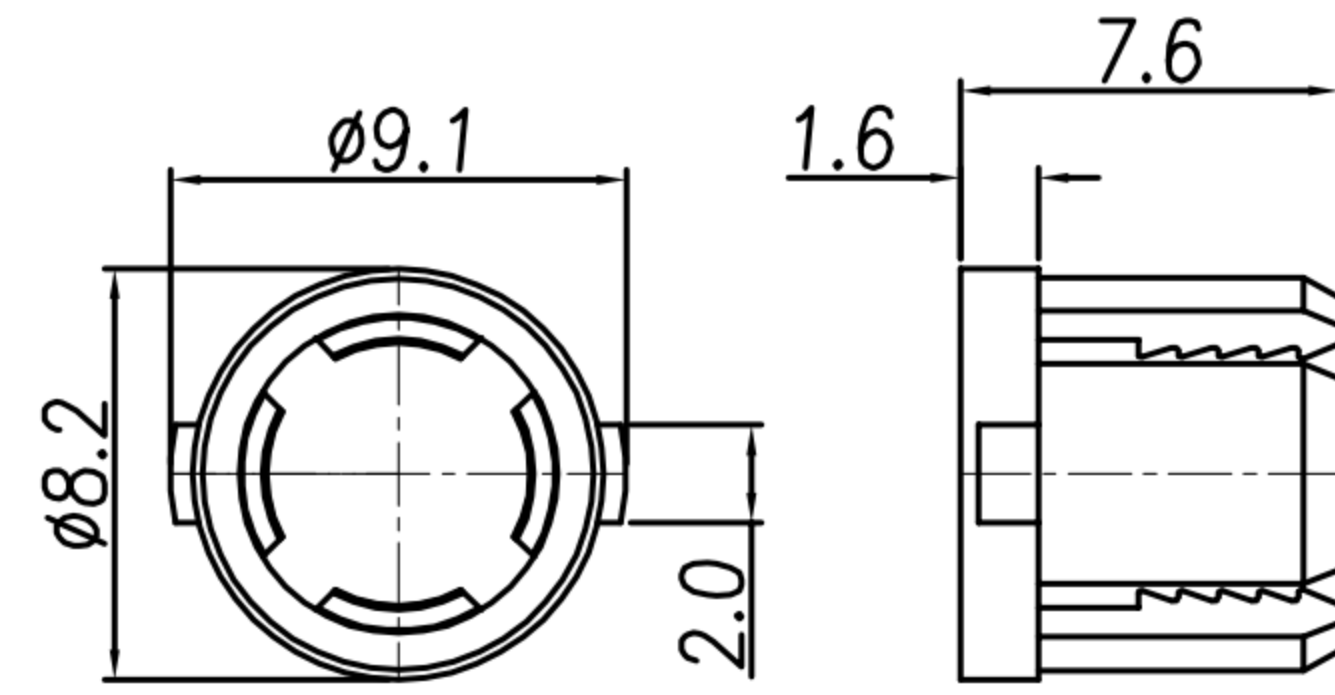
BACK SHELL+SHIELDING+O-RING2
